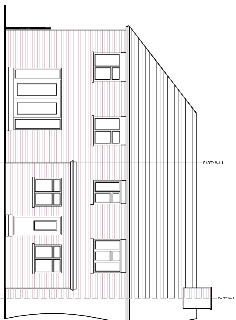
PROPOSED REAR FACING EAST ELEVATION
