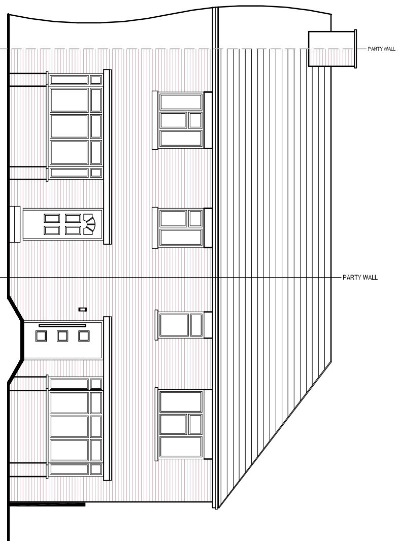
PROPOSED FRONT FACING WEST ELEVATION
